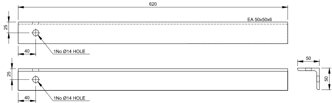
TPB-BR-1 - EA50x50x6 Scale 1:5
