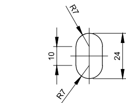
SLOTTED HOLE DETAIL Scale 1:2
