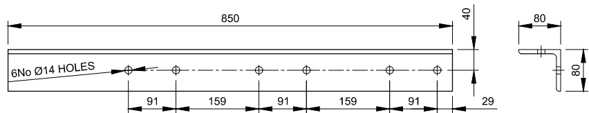
TPL-A-1 - EA 80x80x8 Scale 1:10
