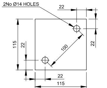
TPL-1 - 10mm THICK Scale 1:5
