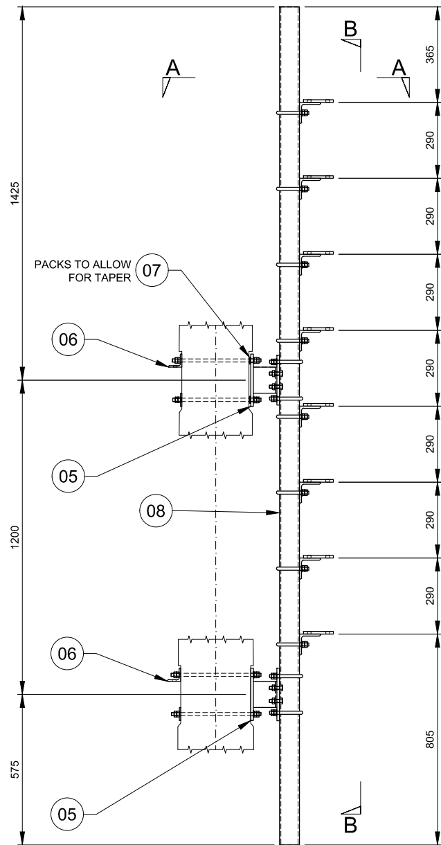
DETAIL G - Tx ANTENNA MOUNT Scale 1:20
