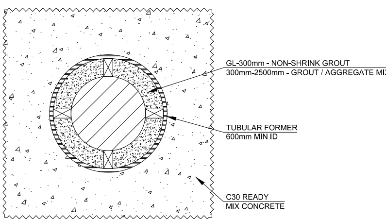
POROPOSED INSTALLATION PLAN VIEW Scale 1:20
