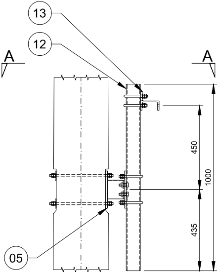
DETAIL H - Rx ANTENNA MOUNT Scale 1:20
