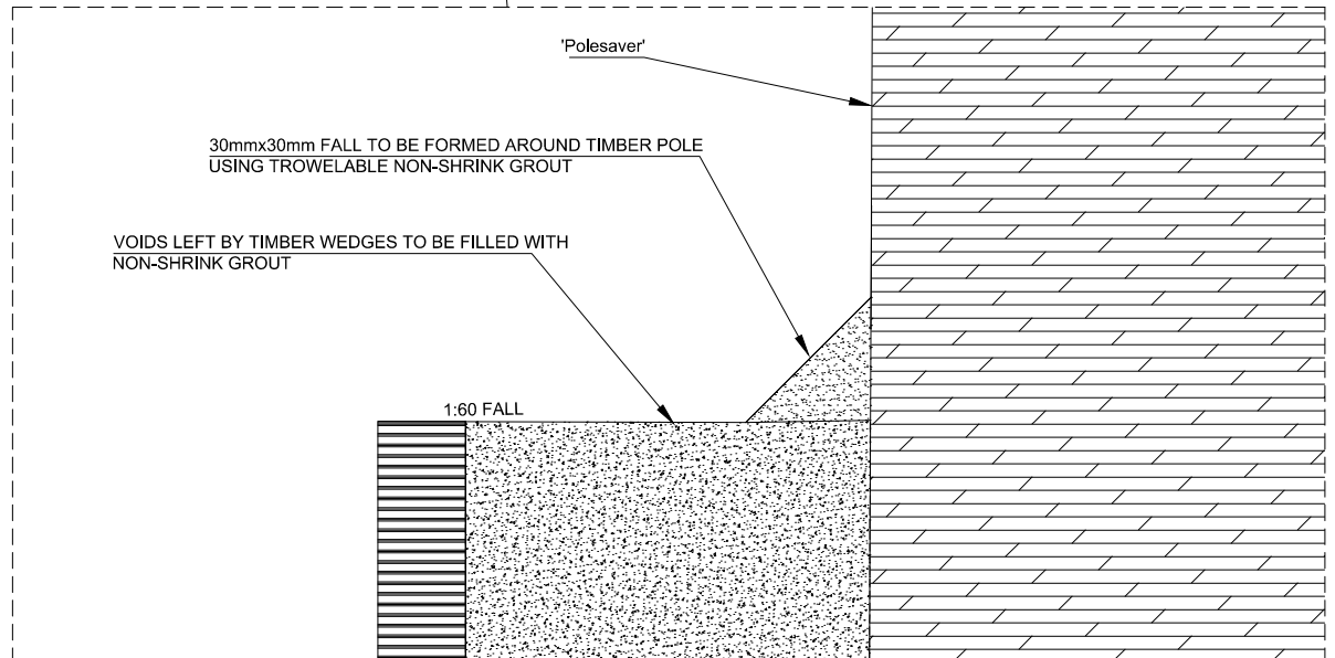
ENLARGED DETAIL Scale 1:2
