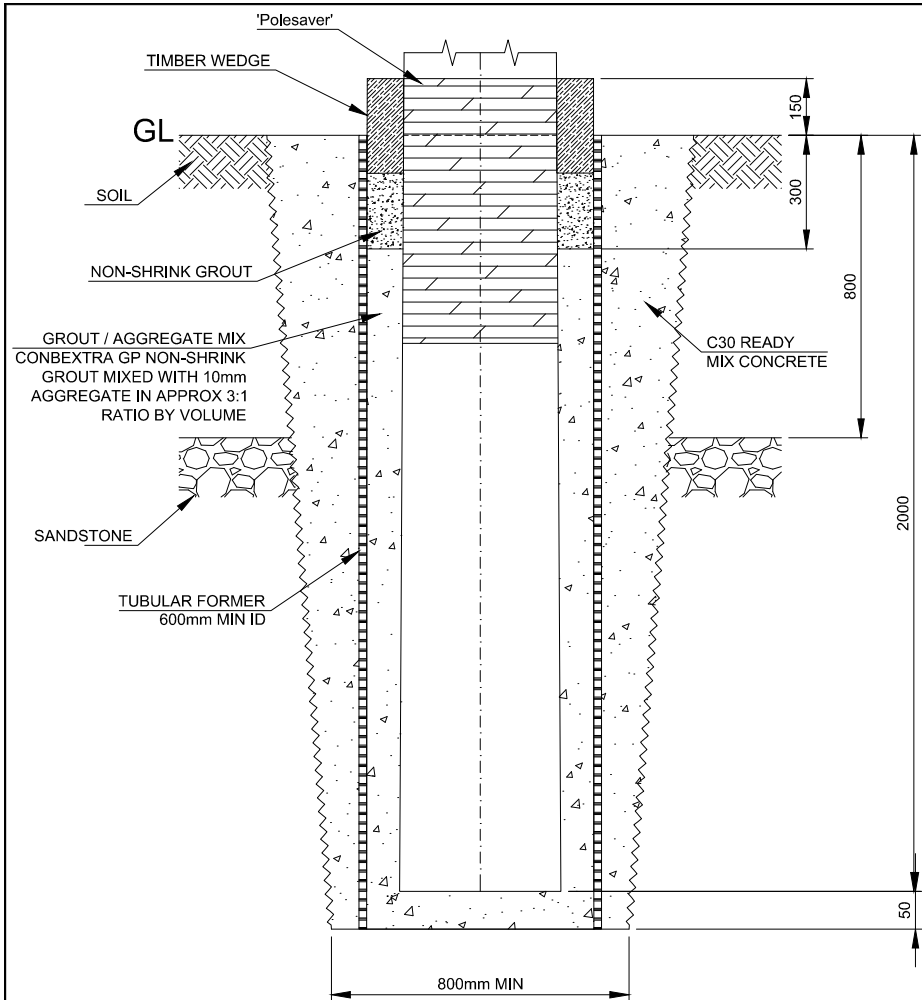
POROPOSED INSTALLATION ELEVATION Scale 1:20
